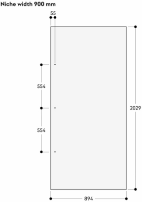
The door panel thickness is 19 mm The maximum door panel dimensions are based on a clearance of 3 mm, based on a single niche Measurements in mm
