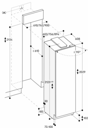
A: Electrical connection Maximum door panel dimensions are based on a clearance of 3 mm The height of the plinth can be reduced to 50 mm Measurements in mm
