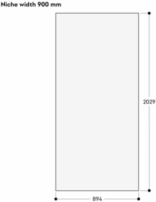
The door panel thickness is 19 mm The maximum door panel dimensions are based on a clearance of 3 mm, based on a single niche Measurements in mm
