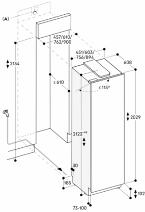
A: Electrical connection Maximum door panel dimensions are based on a clearance of 3 mm The height of the plinth can be reduced to 50 mm Measurements in mm
