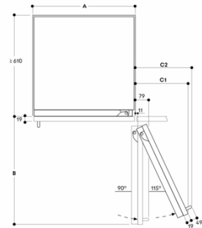
Wall clearance RVB / RVC / RVF / RVH
