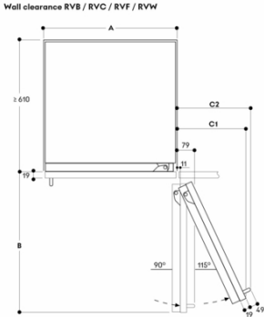
The door panel thickness is 19 mm The maximum door panel dimensions are based on a clearance of 3 mm, based on a single niche Measurements in mm
