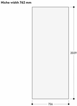
The door panel thickness is 19 mm The maximum door panel dimensions are based on a clearance of 3 mm, based on a single niche Measurements in mm
