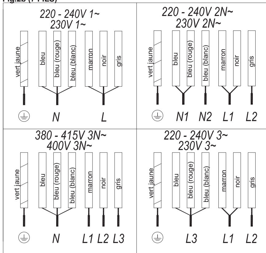
Fig.2b (7 FILS)
